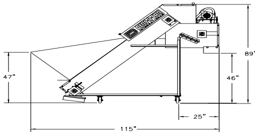
OPTIONAL 2/3 CUBIC YARD HOPPER
