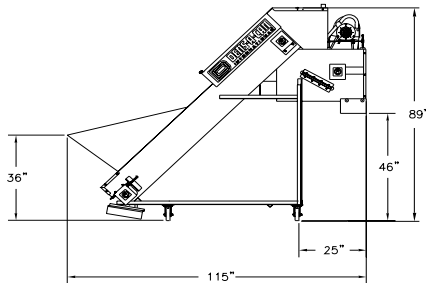
STANDARD 1/3 CUBIC YARD HOPPER
