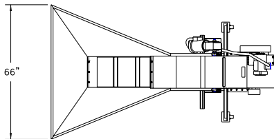
STANDARD 1/3 CUBIC YARD HOPPER
